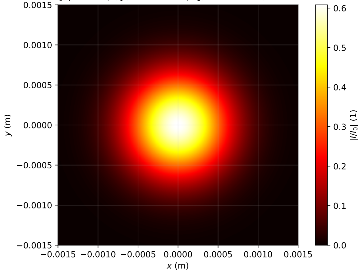
Intensity profile I(x, y, z = 1.751m)/I_0 , Pin=0.1Pcr, artificial time
